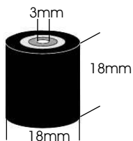
VP-0023 PINCH ROLLER BLV1075A130A
