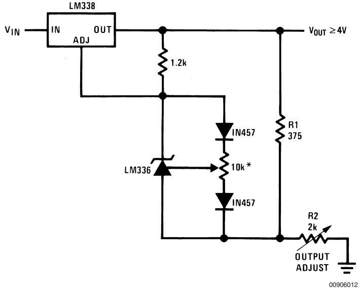
Precision Power Regulator with Low Temperature Coefficient
