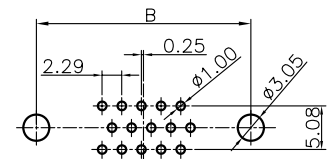
RECOMMEND PCB LAYOUT(TOLERANCE ±0.05) (VIEW FROM TOP SIDE)
