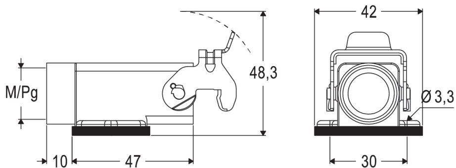
Catalogue drawings
